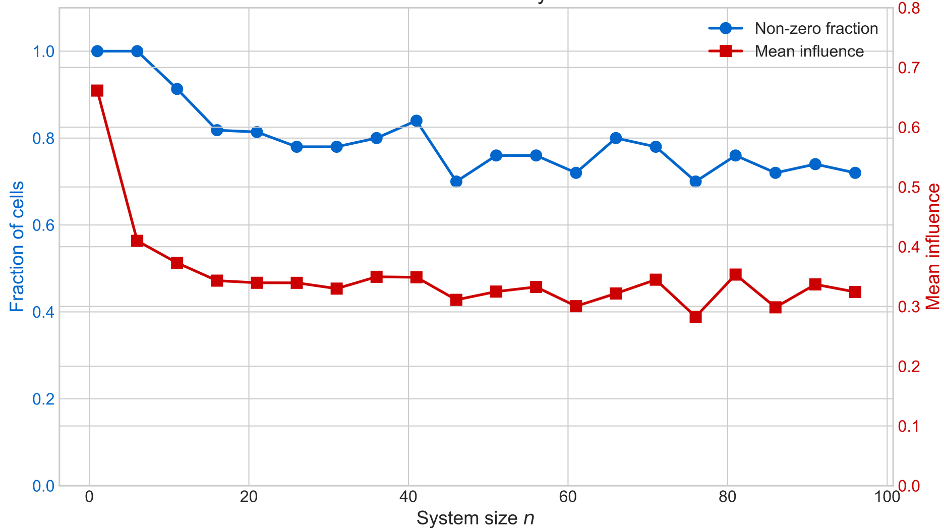
Influence Statistics vs System Size
