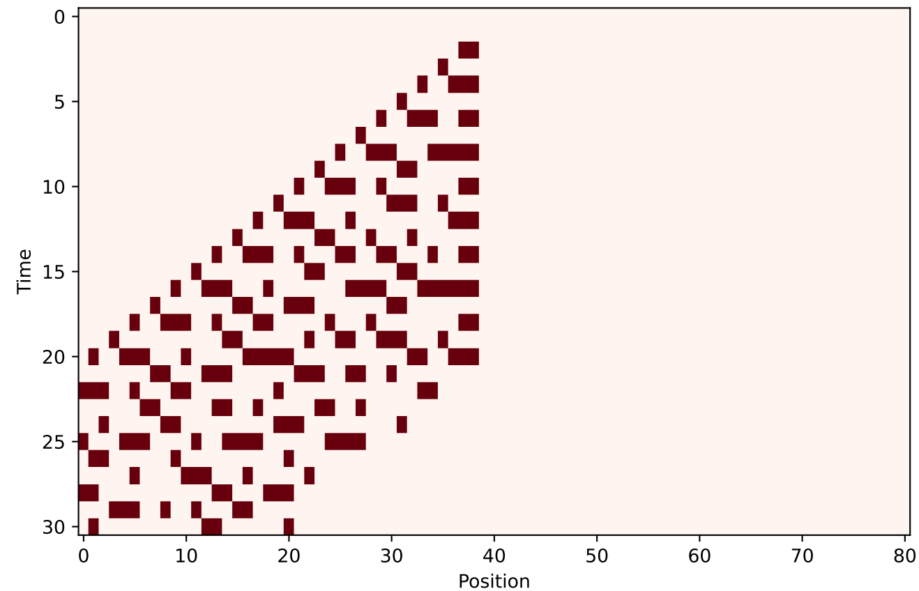
Container Effect Test (Boundary/Interior ratio: 0.49)
