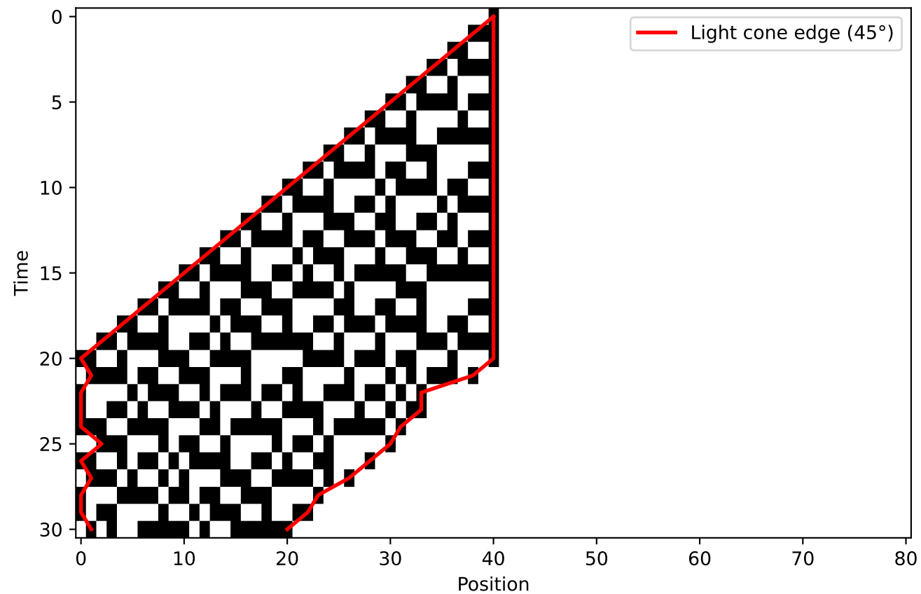
Rule 30 Light Cone (Lattice Gas Container?)
