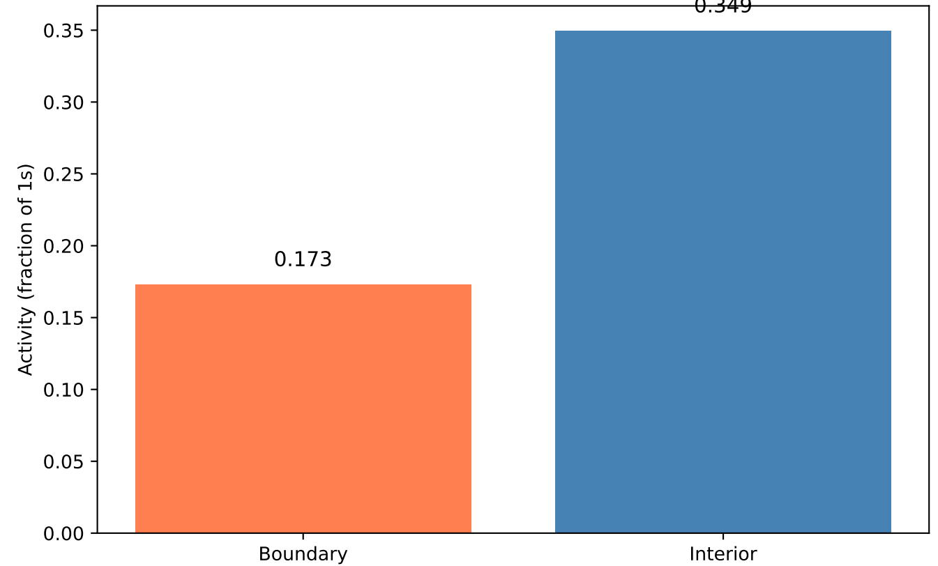
Container Effect Test (Boundary/Interior ratio: 0.49)
