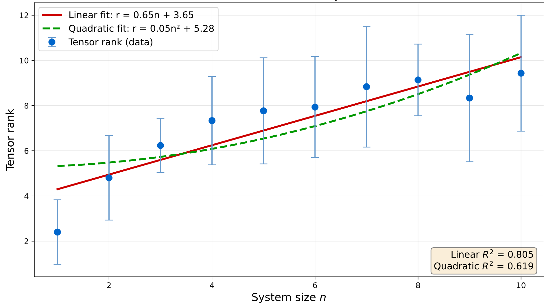
Tensor Rank Growth vs. System Size
