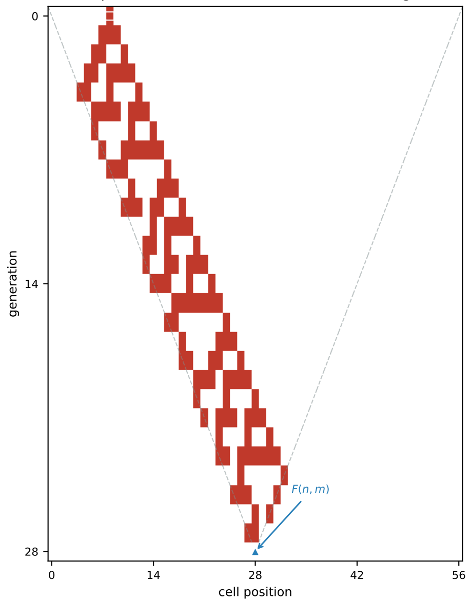
(b) Spike at m = 8 : F(n, m) = leftmost cell at gen n
