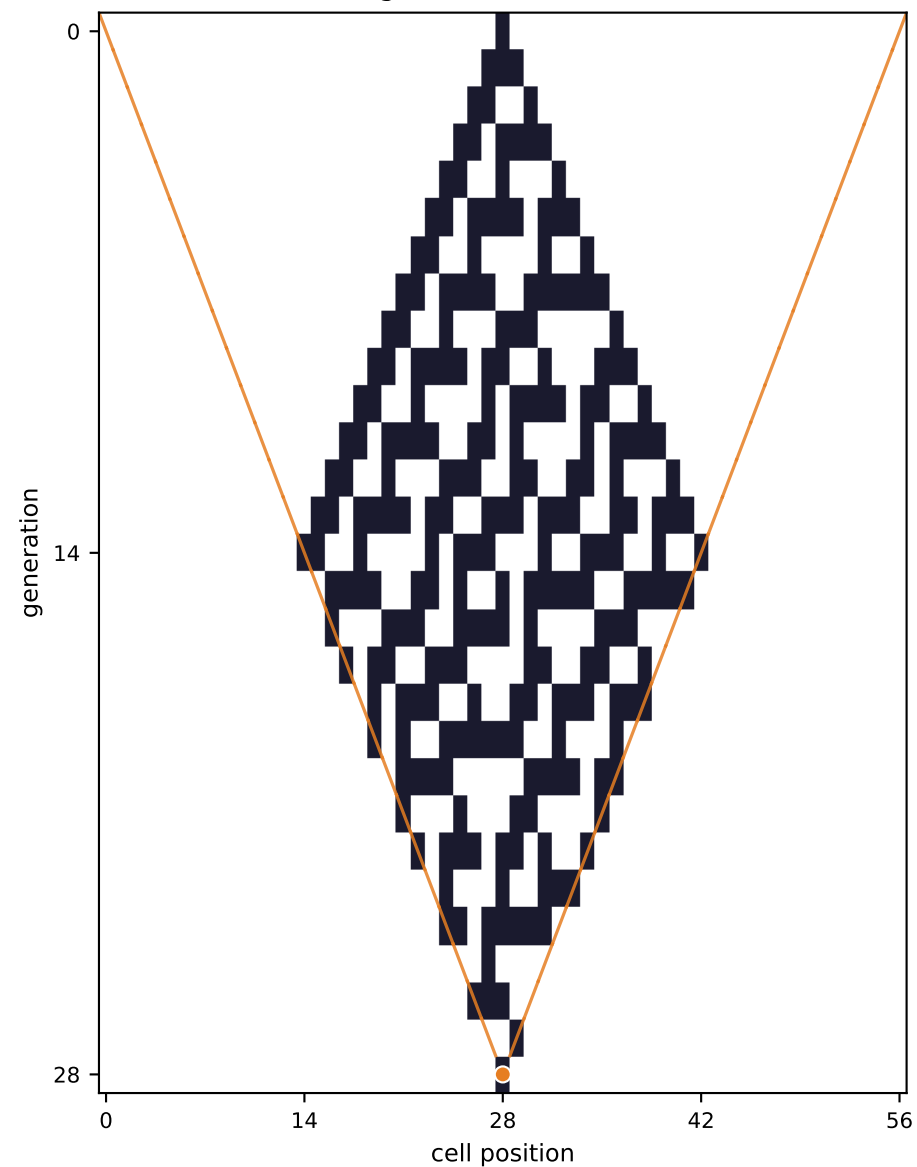
(a) Single black cell e_n , n = 28
