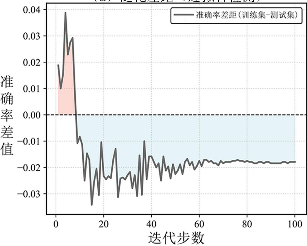
(a) 泛化差距 (过拟合检测)
