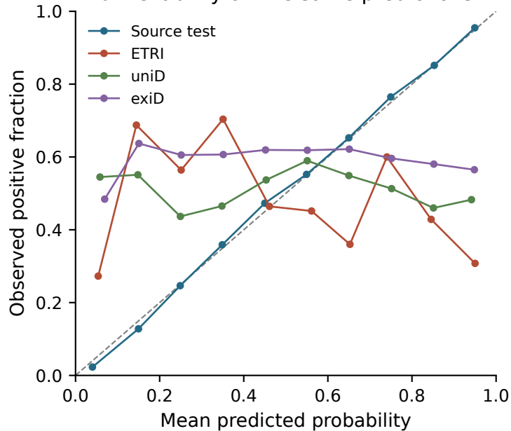
b Reliability on the same predictions
