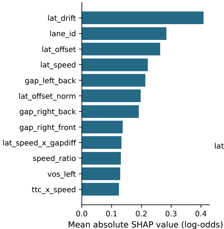
a Source held-out rows
