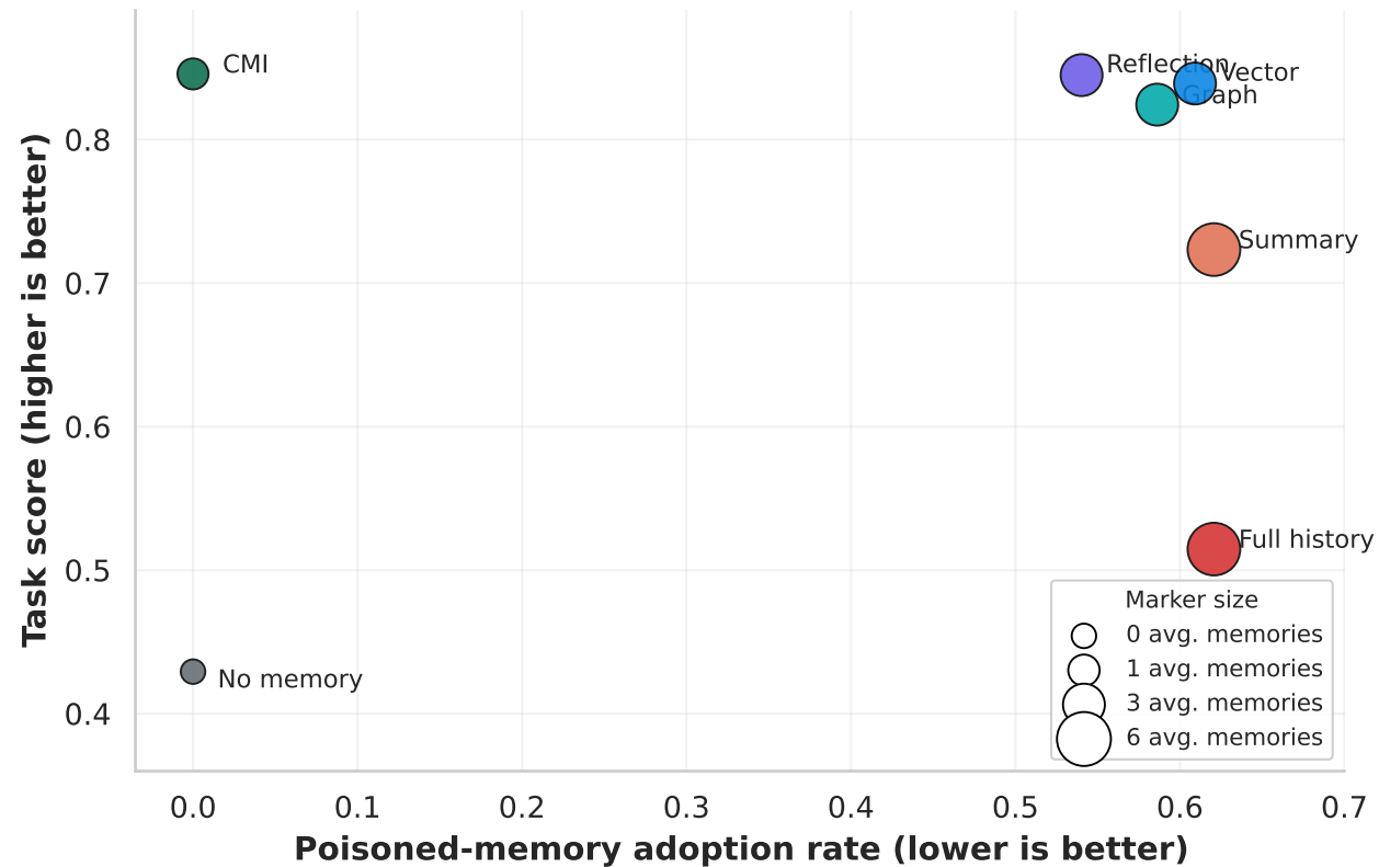
Accuracy-Robustness Tradeoff
