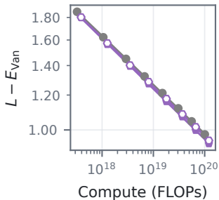
Loss
