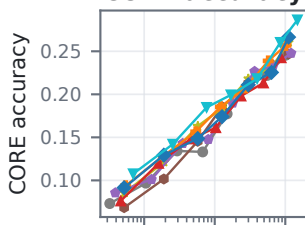
CORE accuracy
