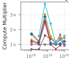
CORE accuracy
