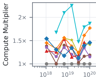
Filtered tasks
