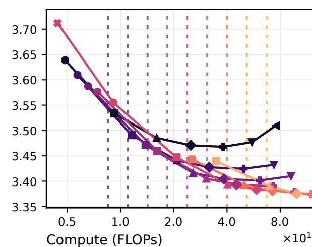
100M × 10 optima
