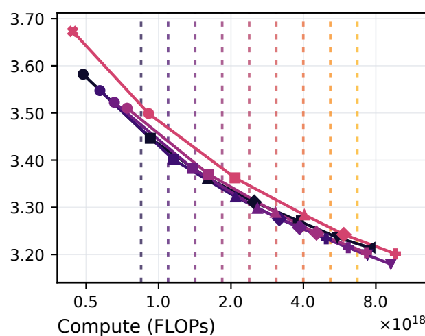
250M × 4 optima
