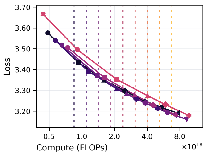
Fresh-data optima
