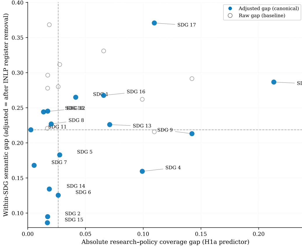
Figure 7. Coverage gap vs semantic gap, one point per SDG. Solid blue points show the adjusted (canonical) gap after register removal; open grey points show the raw gap (naive baseline).
