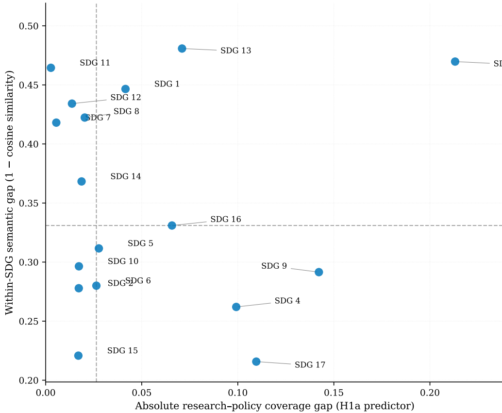
Figure 7. Coverage gap vs semantic gap, one point per SDG.
