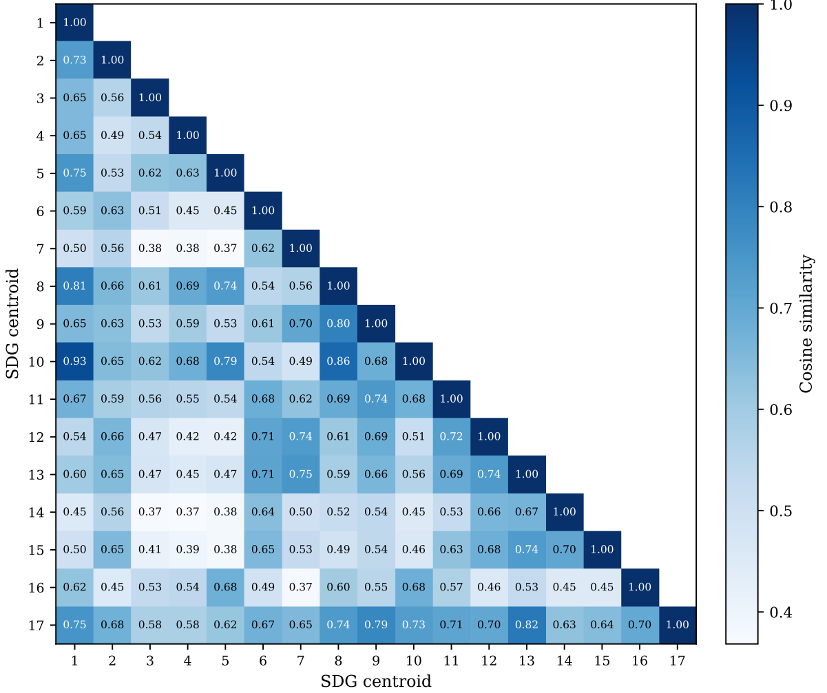
Figure 7. Pairwise cosine similarity between canonical SDG centroids (lower triangle). SDG 13 and SDG 17 sit close together (cosine 0.821), as do SDGs 1, 8, and 10.
