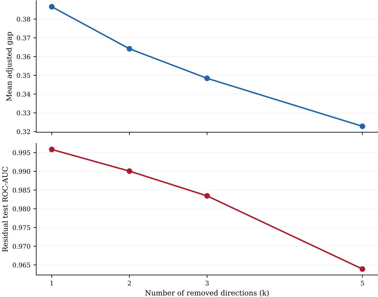
Additional register-confidence checks: multi-direction subtraction sensitivity
