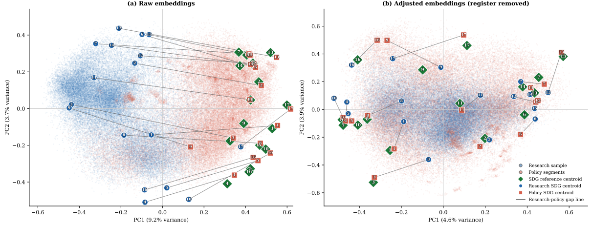
Figure 4. PCA before/after INLP register removal (MPNet). (a) Raw embeddings: research and policy clouds are separated. (b) Adjusted embeddings (register removed via INLP): the clouds merge, confirming that the raw separation is driven by register rather than topic. Each panel fits PCA on its respective data; panels have independent axes. Descriptive projection only; all reported distances remain in the original embedding space.
