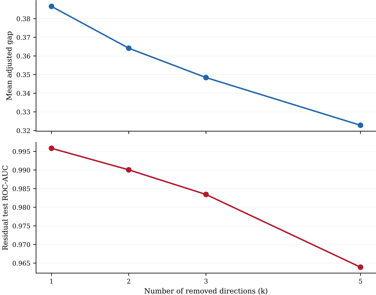
Additional genre-confidence checks: multi-direction subtraction sensitivity
