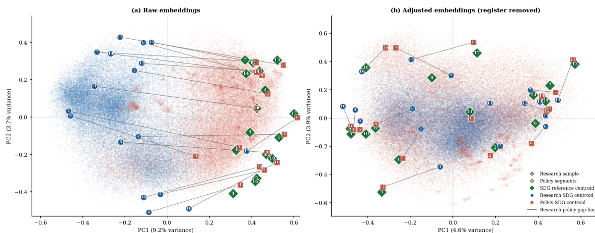
Figure 4. PCA before/after INLP register removal (MPNet).
