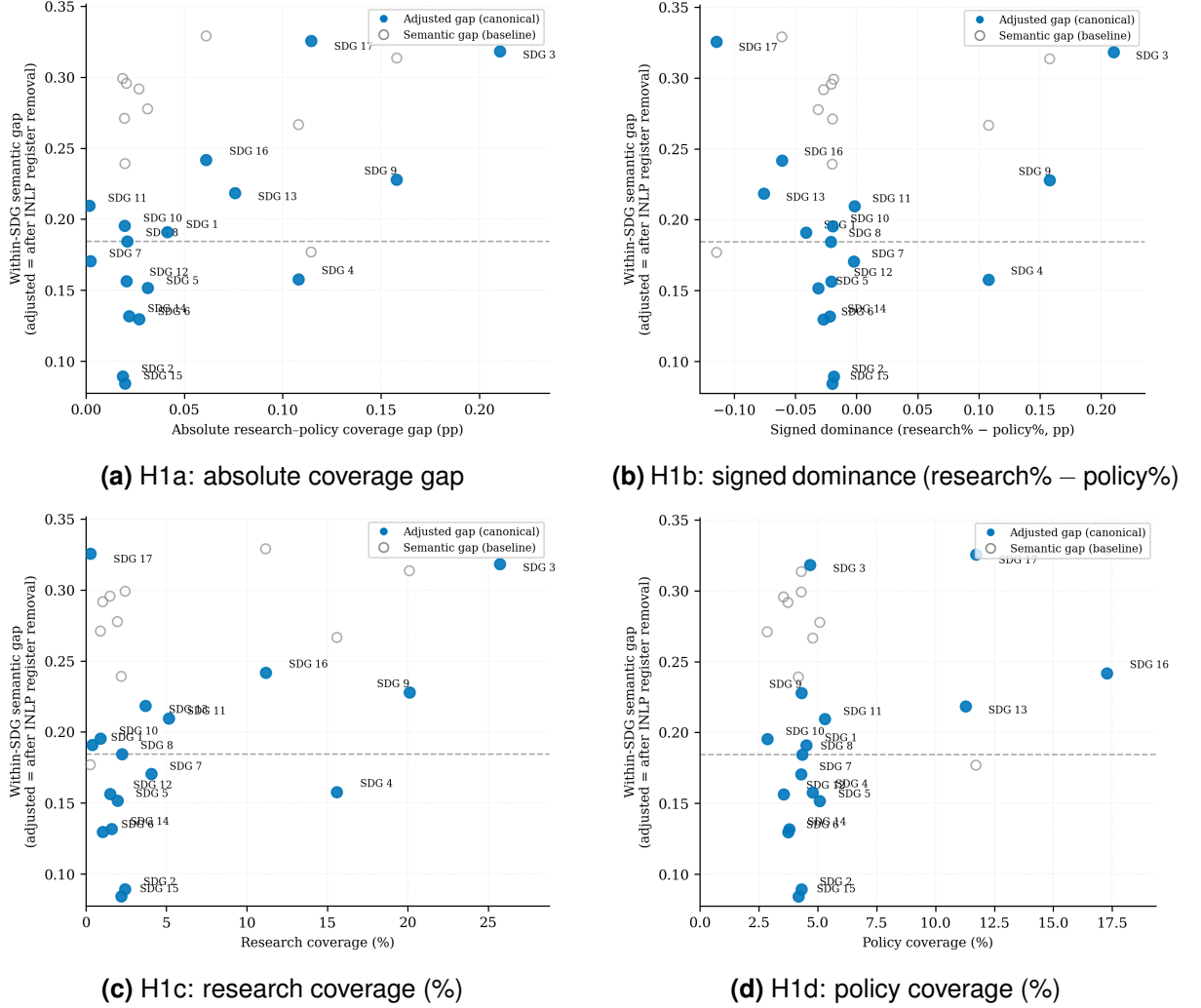
Figure 6. Coverage predictor vs within-SDG semantic gap, one point per SDG.
