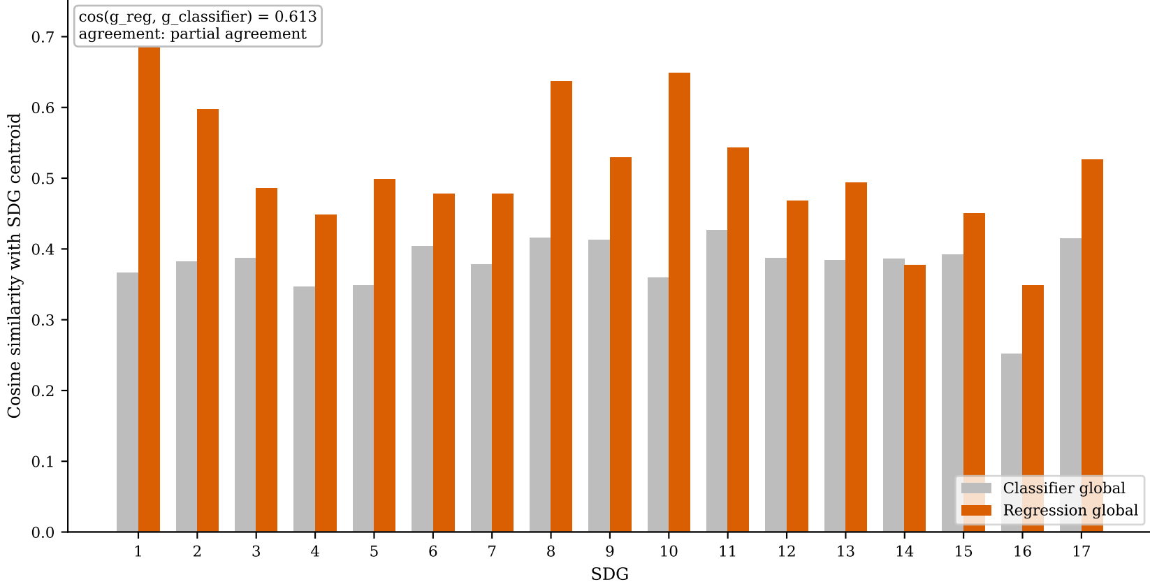
Classifier vs regression register-direction alignment
