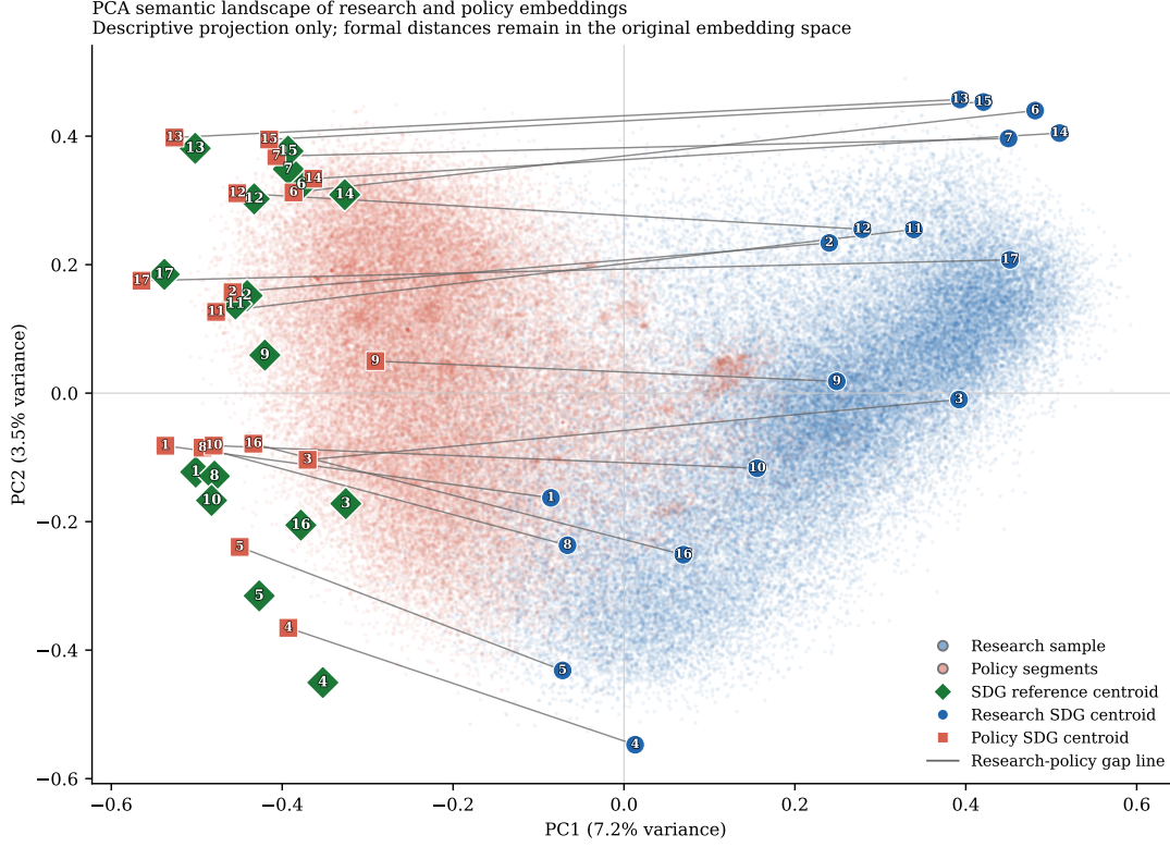
Figure 1. PCA semantic landscape of the combined research-policy embedding space. Background points show a balanced research-policy sample used to fit and visualise the two-dimensional projection. Diamond markers show the 17 SDG reference centroids; circle and square markers show the full-corpus research and policy SDG centroids, with thin segments linking each pair. The projection is descriptive only; formal semantic distances are computed in the original embedding space.
