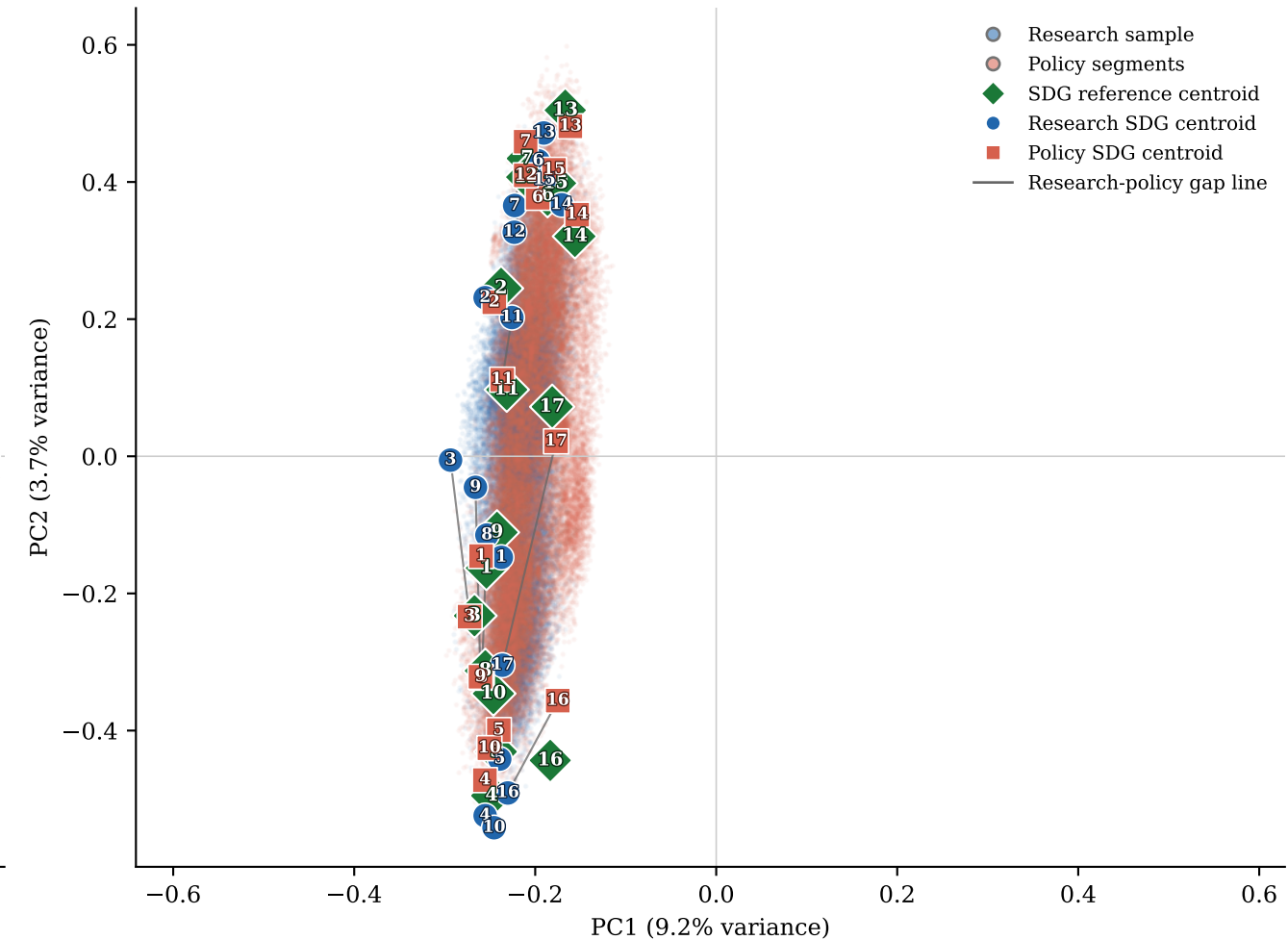
(b) Adjusted embeddings (register removed)
