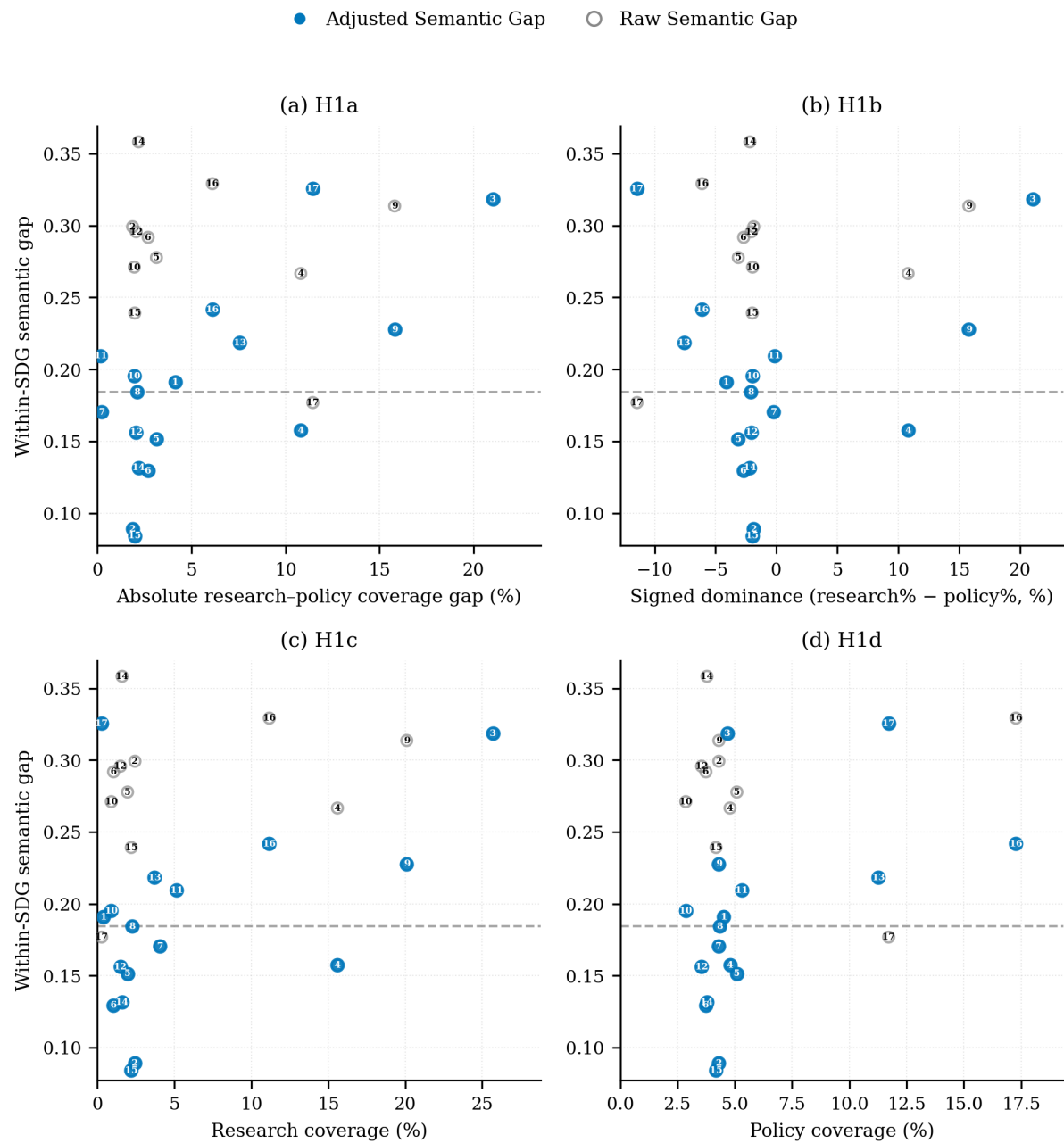
Figure 6. Coverage predictor vs within-SDG semantic gap, one point per SDG.
