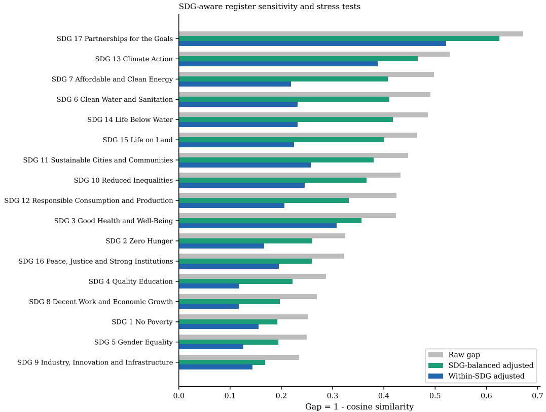
Figure 8. Raw semantic gap compared with SDG-aware register procedures. The green bars show the SDG-balanced global sensitivity check. The blue bars show the within-SDG stress test, which is more prone to over-subtraction.
