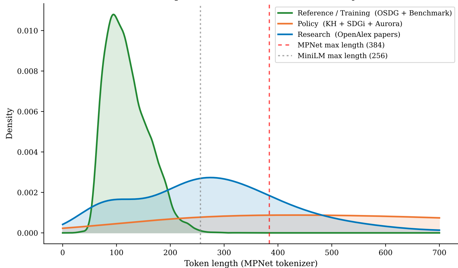
Token-length distribution across dissertation corpora
