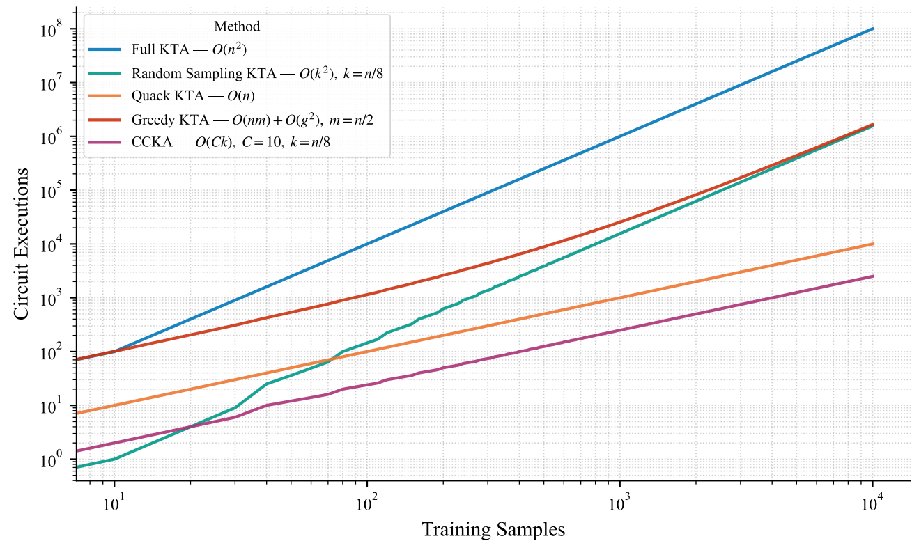
Circuit Executions Across KTA Methods by Training Samples
