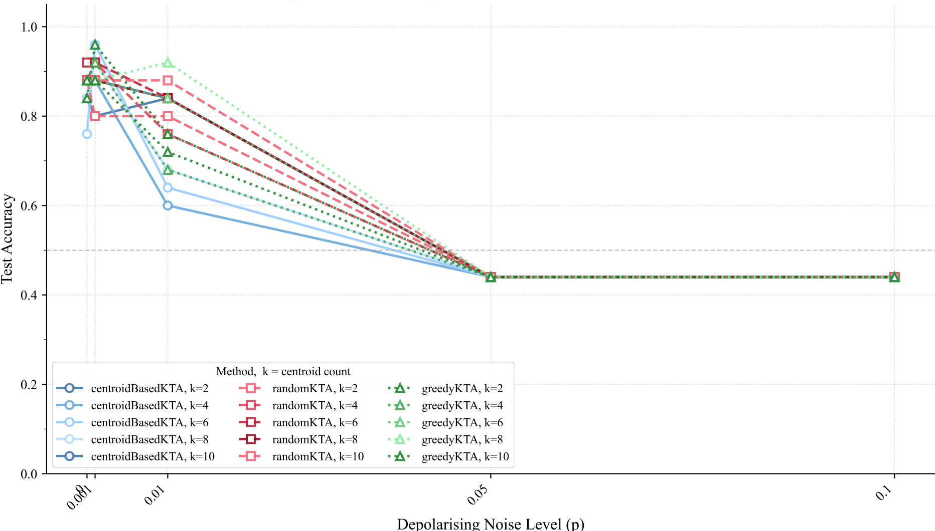
Test Accuracy vs. Noise Level by Method & Centroid Count — Corners Dataset
