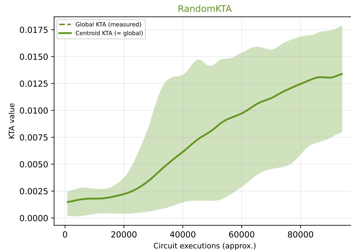
Experiment 1: Centroid-Space KTA vs Global KTA — checkerboard (mean \pm min/max, 10 seeds)
