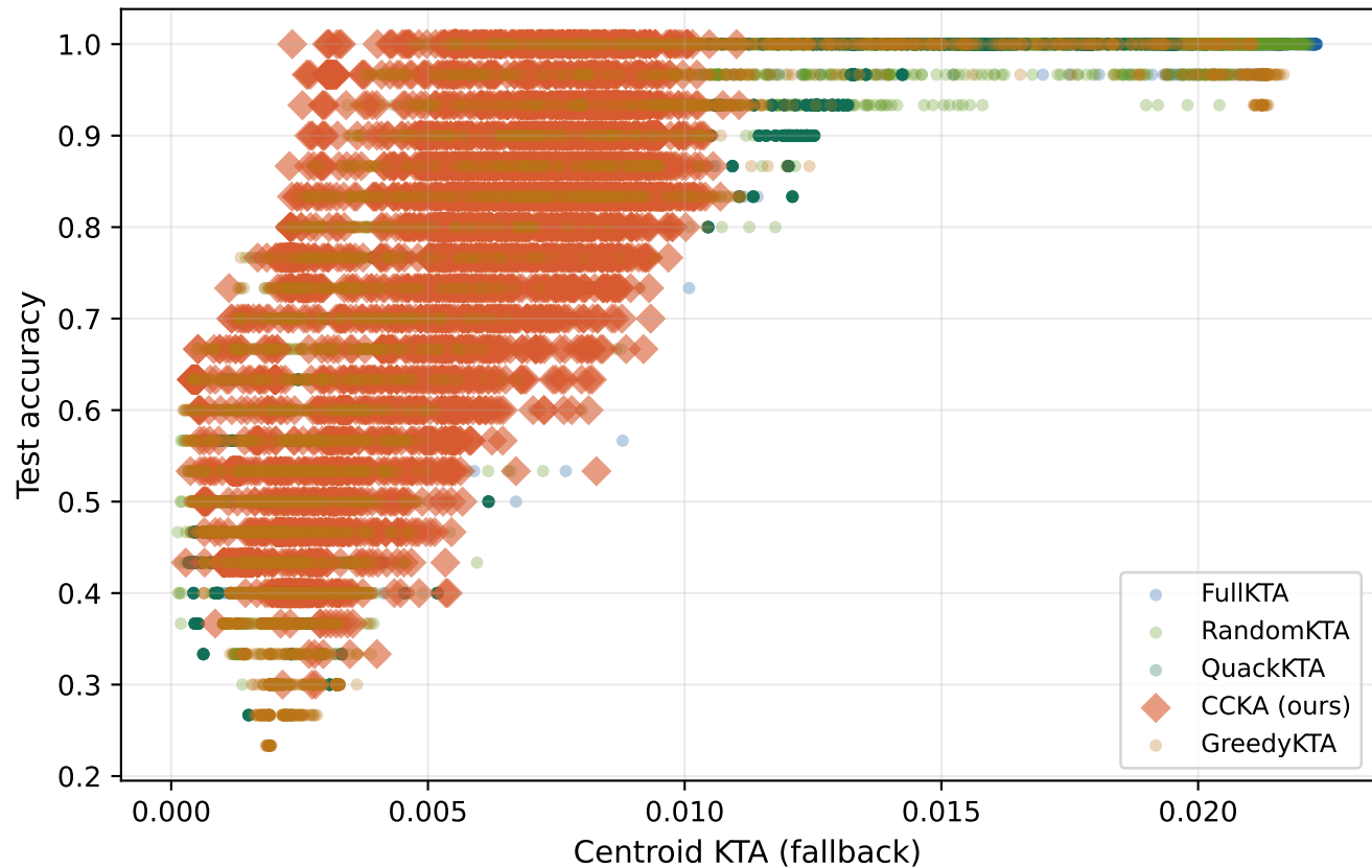
Centroid KTA vs test accuracy checkerboard (all 10 seeds pooled)
