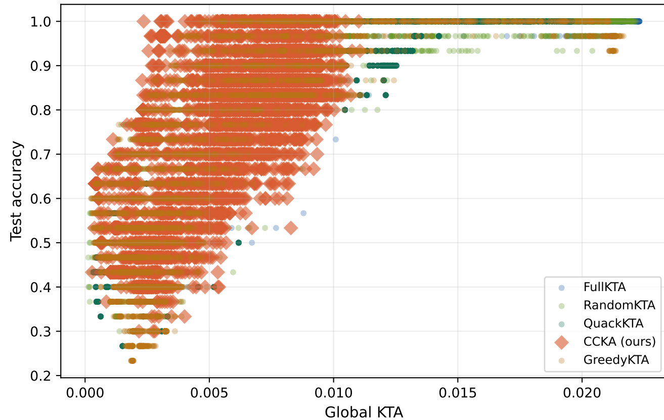
Global KTA vs test accuracy checkerboard (all 10 seeds pooled)
