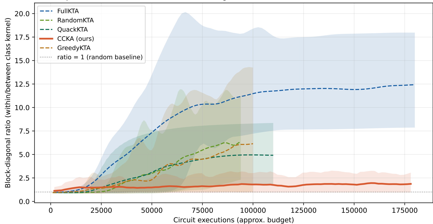
Experiment 2: Kernel block structure vs budget — checkerboard (mean \pm min/max, 10 seeds)
