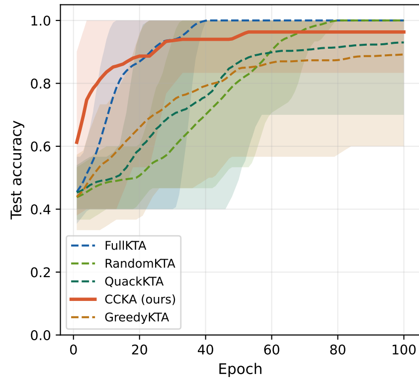
Test accuracy vs epoch — checkerboard (mean \pm min/max, 10 seeds)
