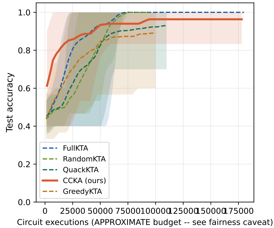
Test accuracy vs budget — checkerboard (mean \pm min/max, 10 seeds)
