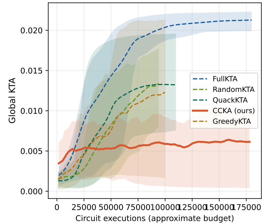
Global KTA vs budget — checkerboard (mean \pm min/max, 10 seeds)
