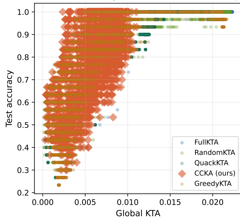
Global KTA vs test accuracy — checkerboard (all 10 seeds pooled)
