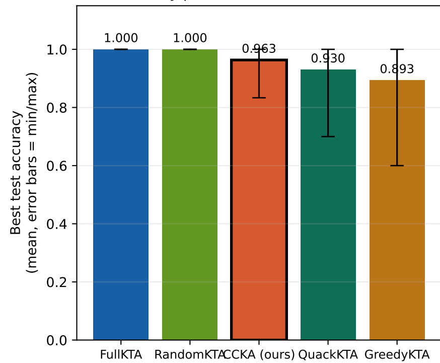
Best test accuracy per method — checkerboard (10 seeds)
