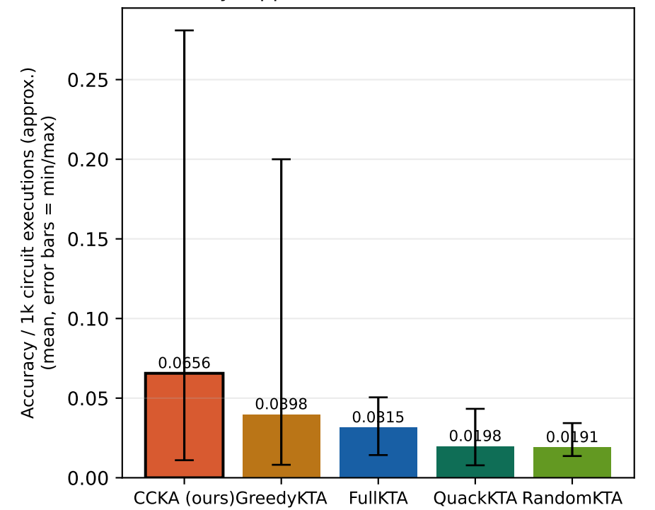
Cost efficiency (approximate) — checkerboard (10 seeds)
