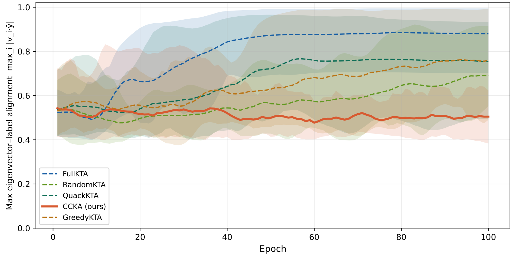
Best-aligned eigenvector over training — checkerboard mean \pm min/max, 10 seeds
