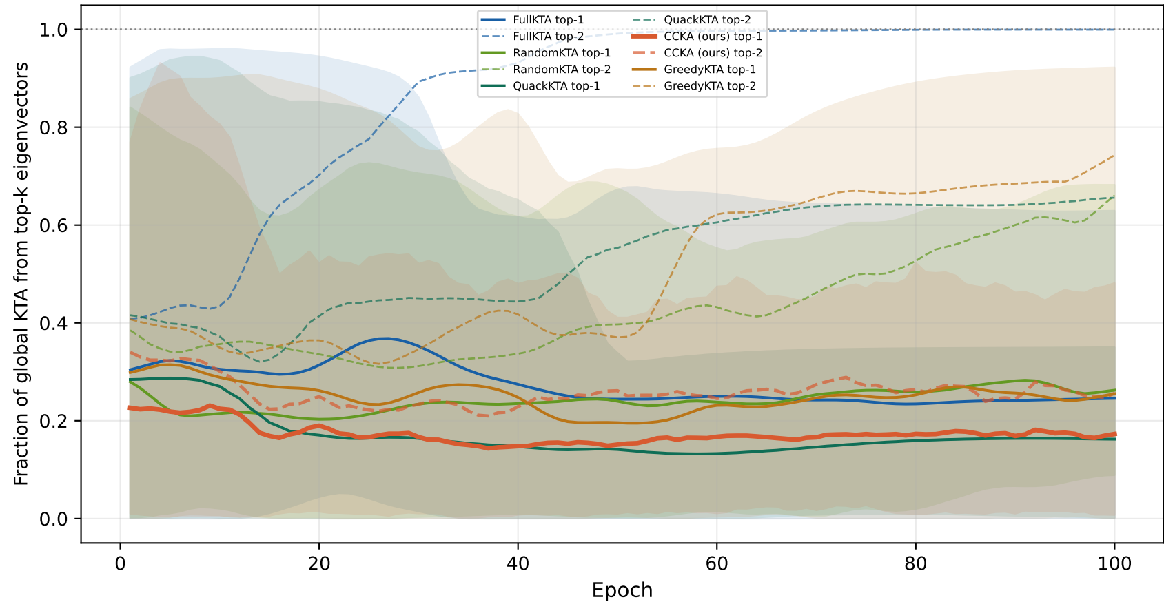
KTA decomposition by rank — checkerboard (mean \pm min/max, 10 seeds)
