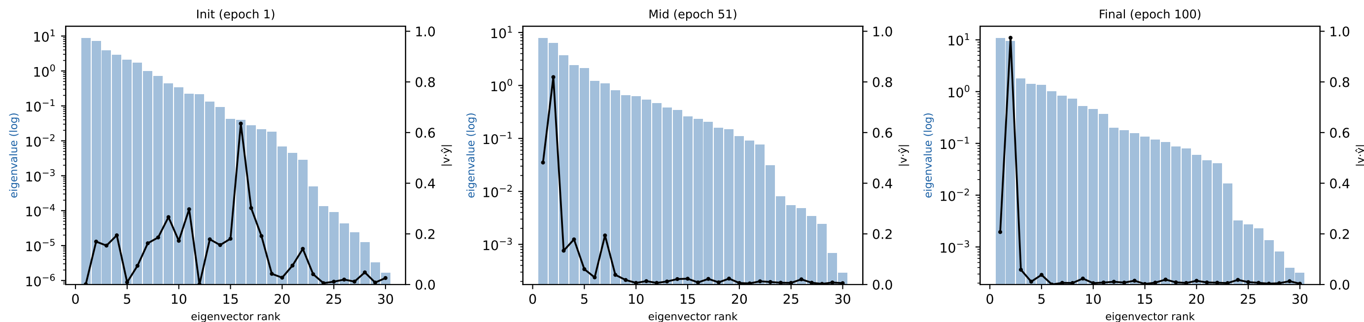
Eigenvalue spectrum + label alignment — checkerboard (seed=0) CCKA: label alignment concentrated in few eigenvectors (low-rank)
