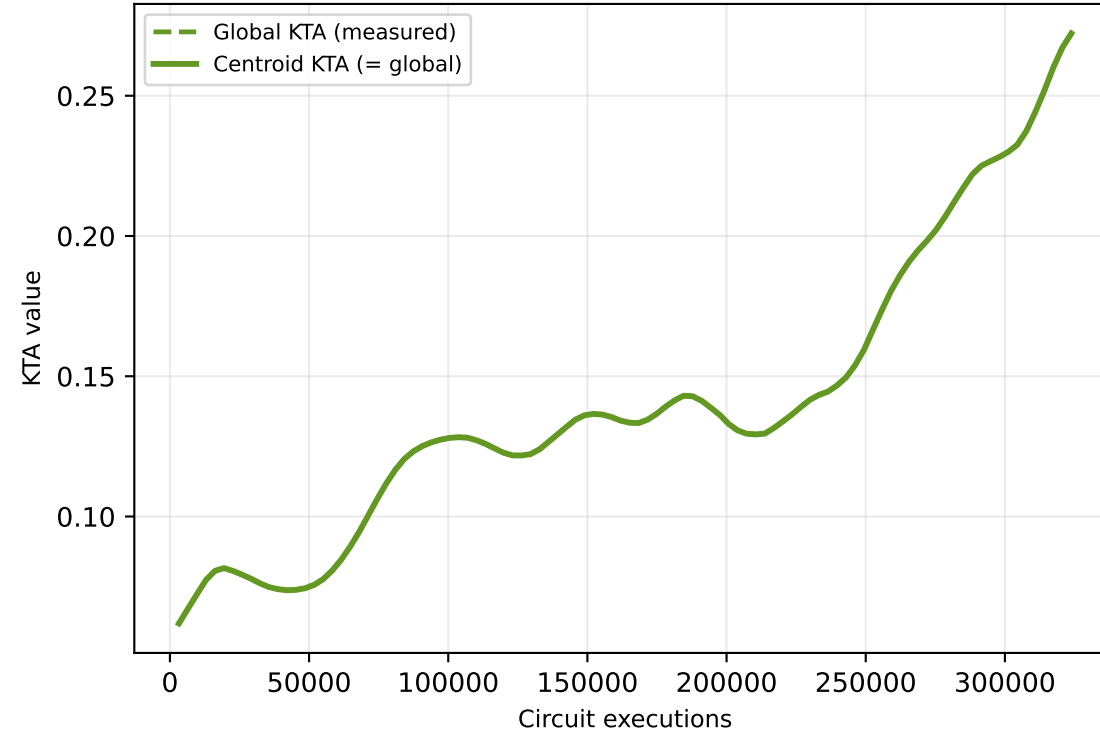
GreedyKTA
