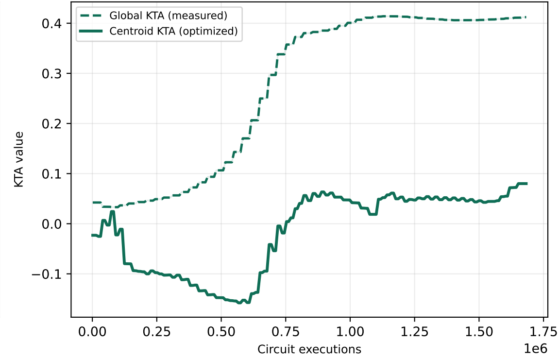
QuackKTA
