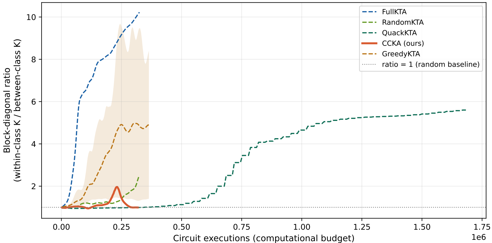
Experiment 2: Kernel matrix block structure vs budget — checkerboard High ratio = clean class separation in kernel space (mean \pm min/max, 5 seeds)
