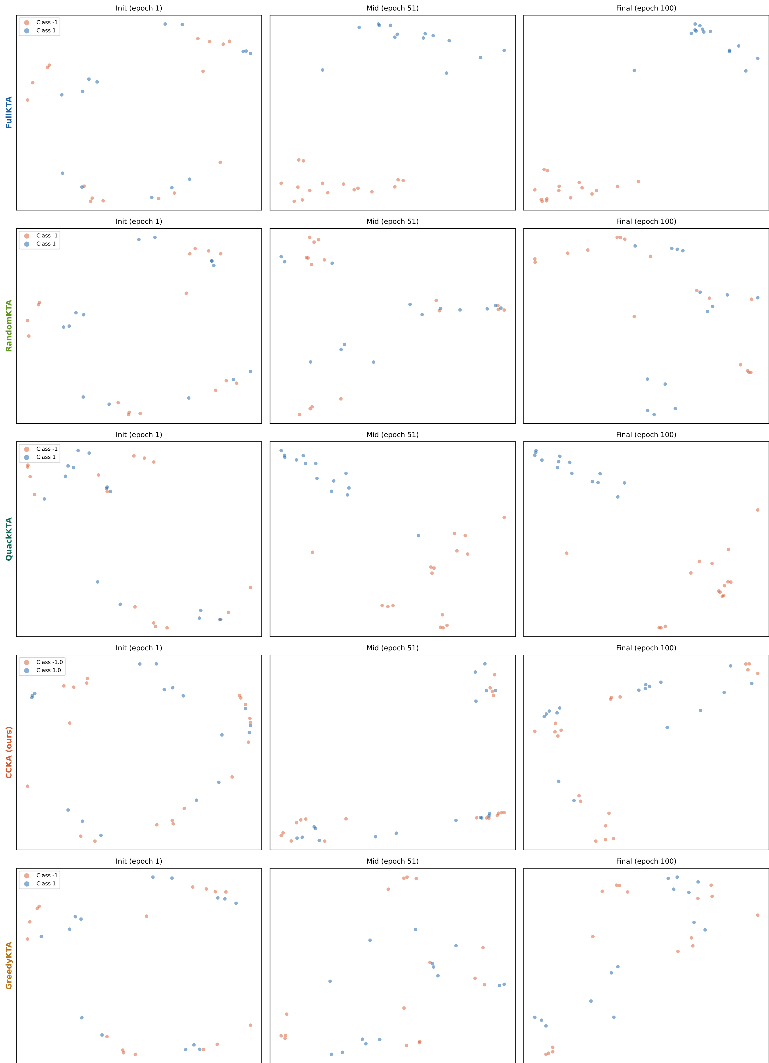
Experiment 4: Kernel PCA embedding snapshots — checkerboard (seed=0) Each row: one method. Columns: init / mid / final epoch. CCKA expected to separate classes earlier and more cleanly.
