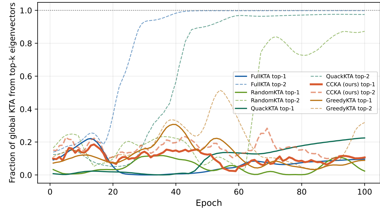
KTA decomposition by rank — checkerboard Near 1.0 = essentially all KTA in the top 1-2 directions (low-rank)
