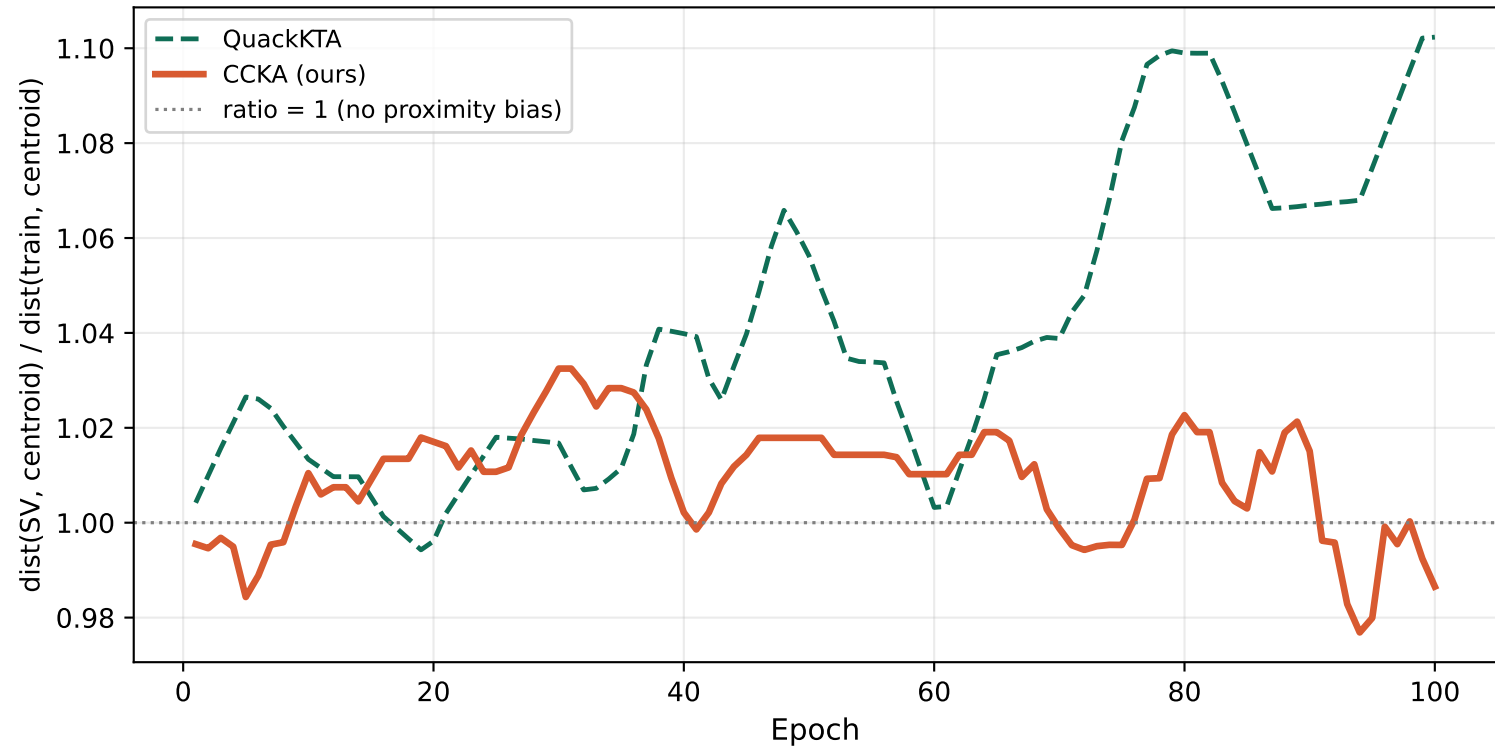
SV-1: Support vector proximity to centroids — checkerboard Ratio < 1 → SVs cluster near centroids (boundary anchoring)
