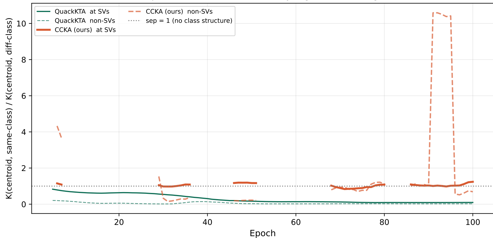
SV-4: Centroid-to-SV kernel separation — checkerboard Solid = at support vectors | Dashed = at non-support-vectors CCKA expected: solid >> dashed (boundary-targeted centroid alignment)
