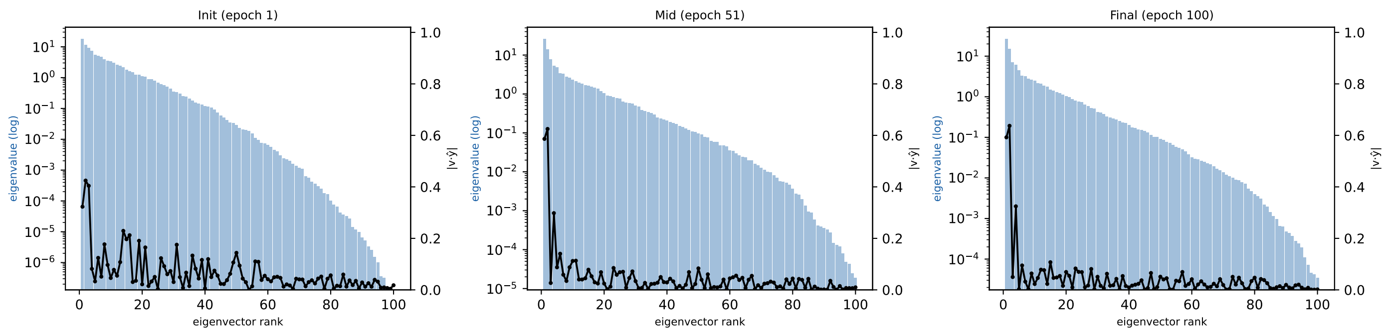
Eigenvalue spectrum (bars) + label alignment (line) — corners CCKA: label alignment concentrated in few eigenvectors (low-rank)
