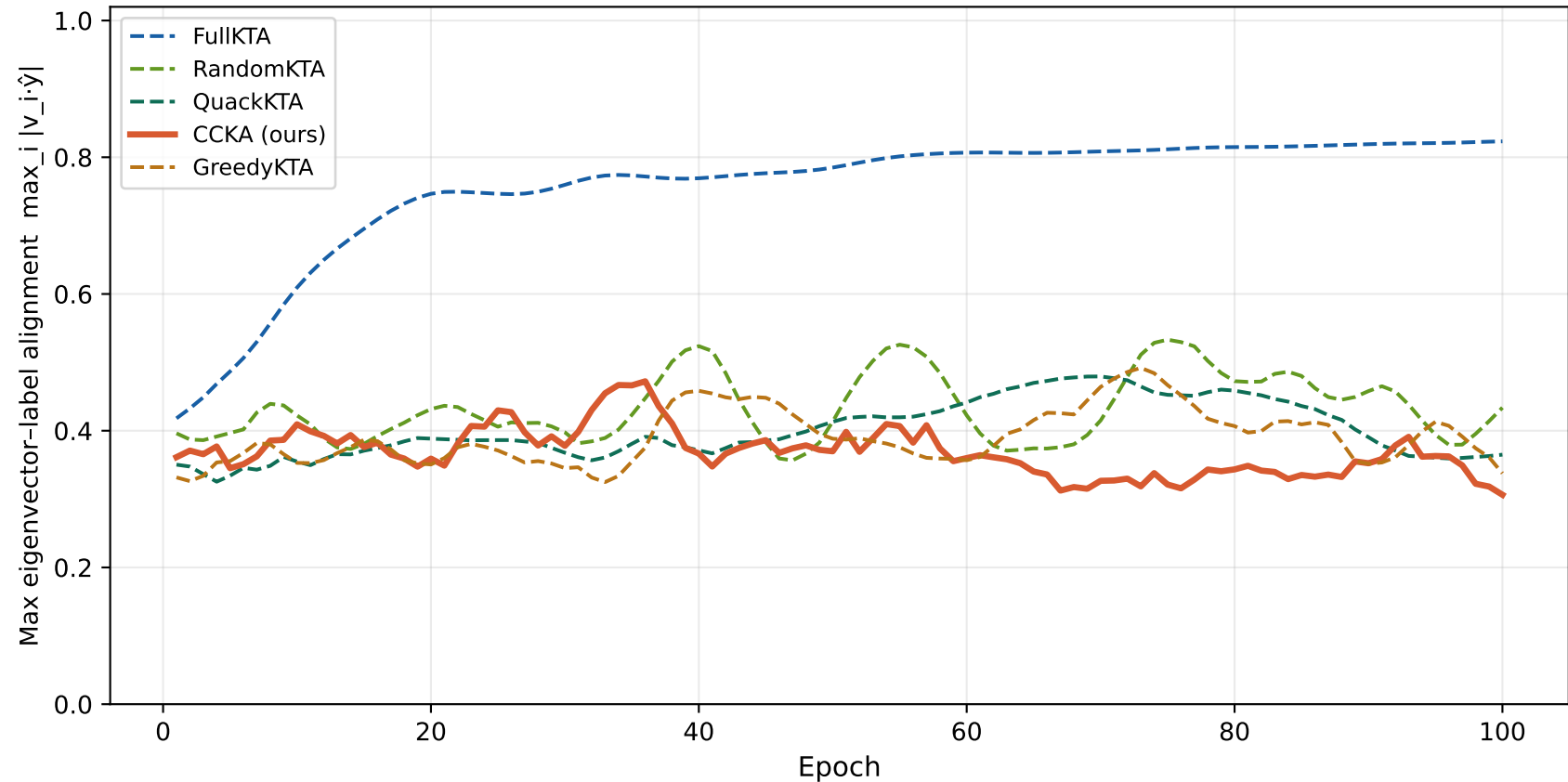
Best-aligned eigenvector over training — donuts CCKA collapse (~ep64) should show a sharp drop here
