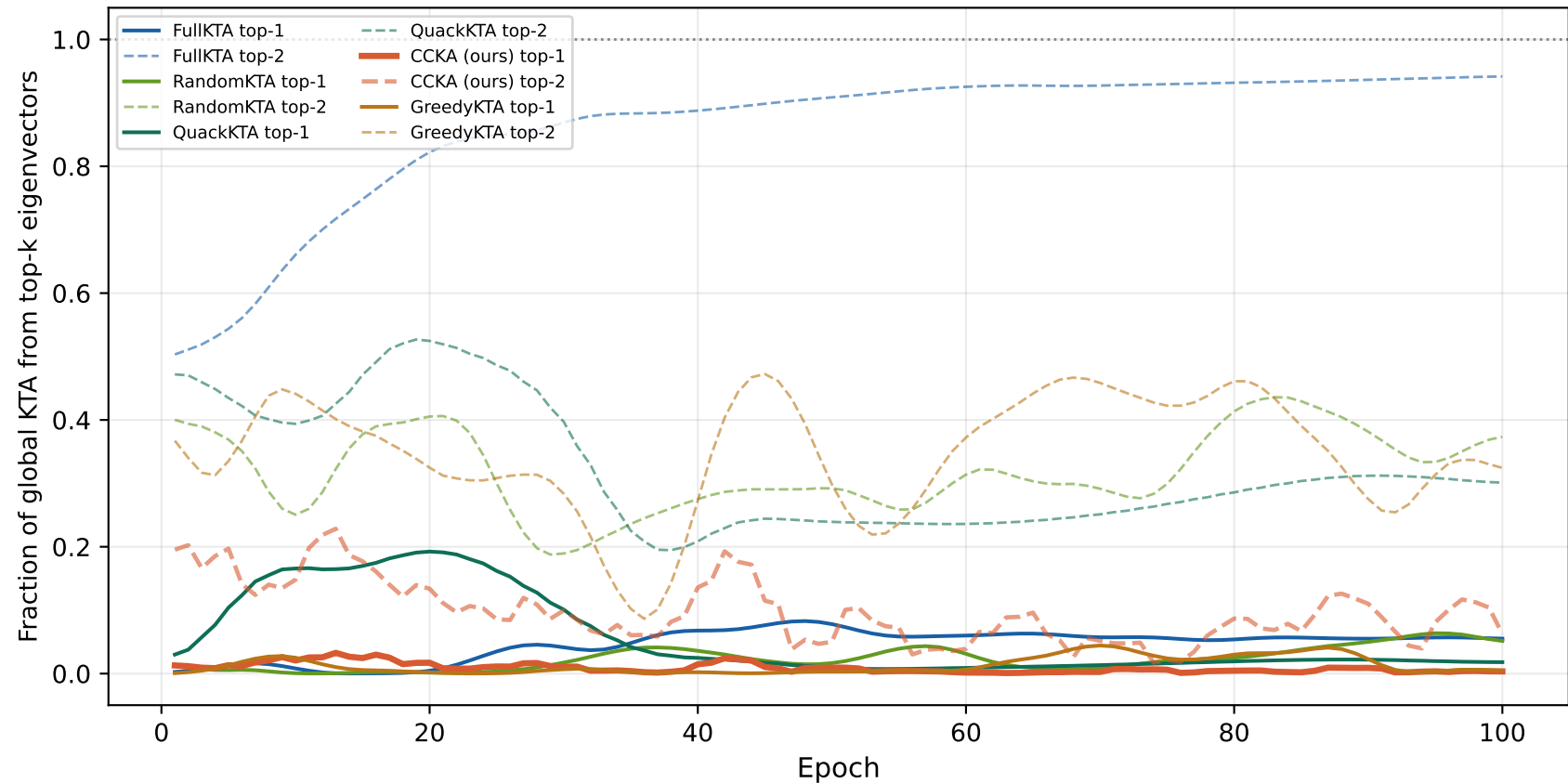
KTA decomposition by rank — donuts Near 1.0 = essentially all KTA in the top 1-2 directions (low-rank)
