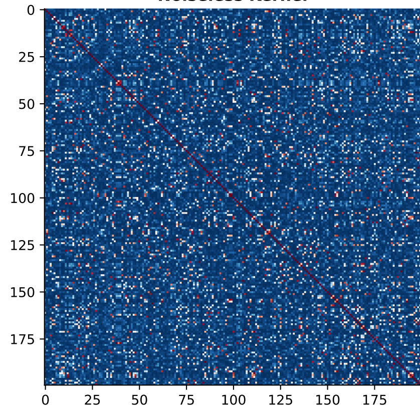
Noiseless Kernel
