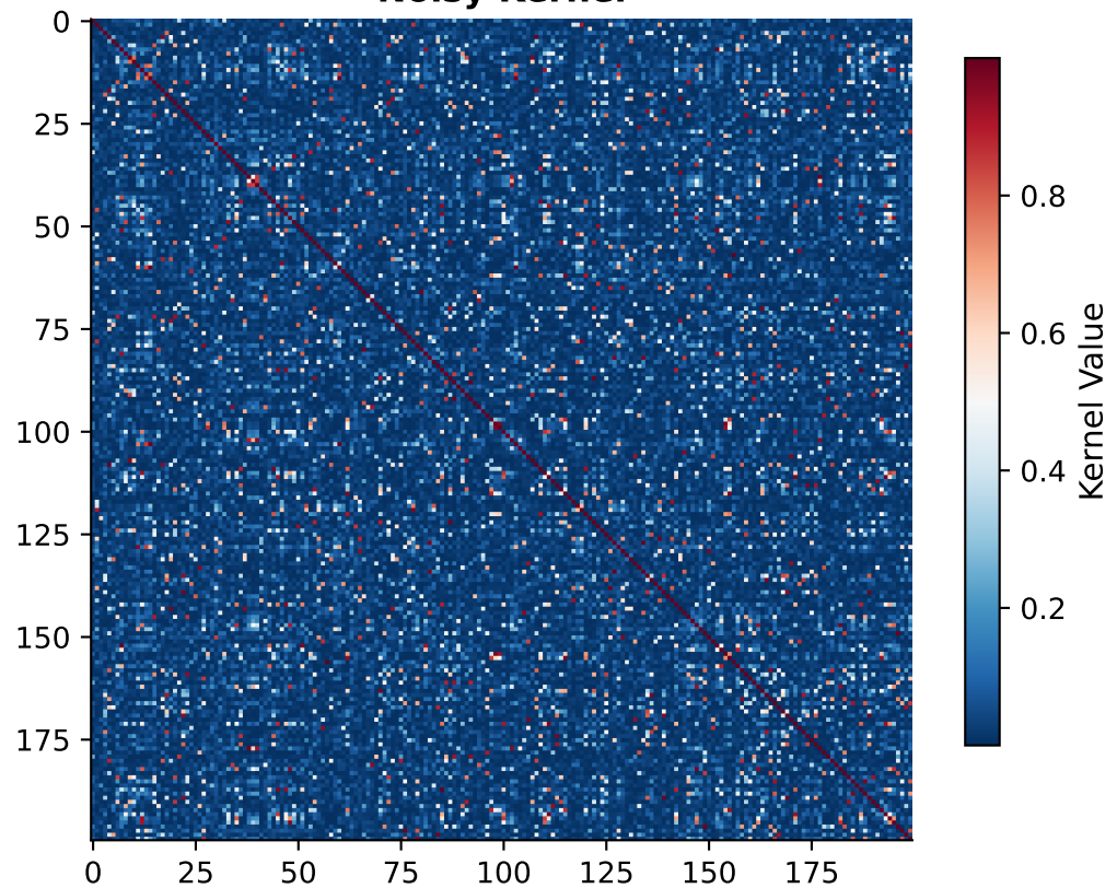
Noisy Kernel
