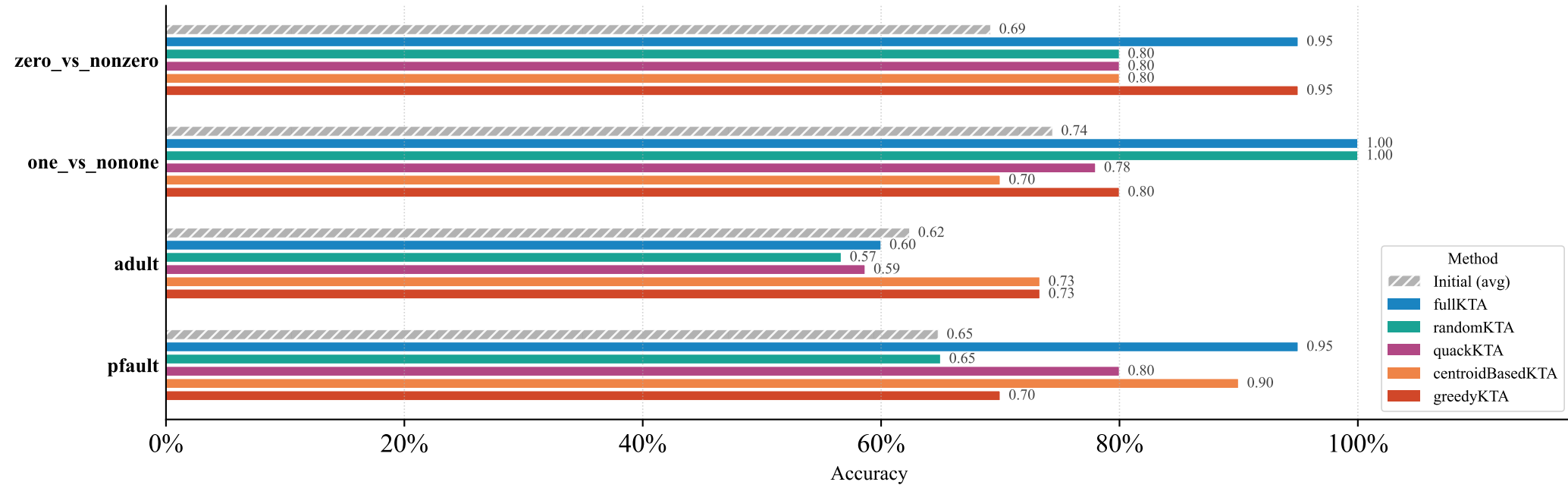
Final Test Accuracy by Dataset & Method (averaged over all iterations and centroid counts)
