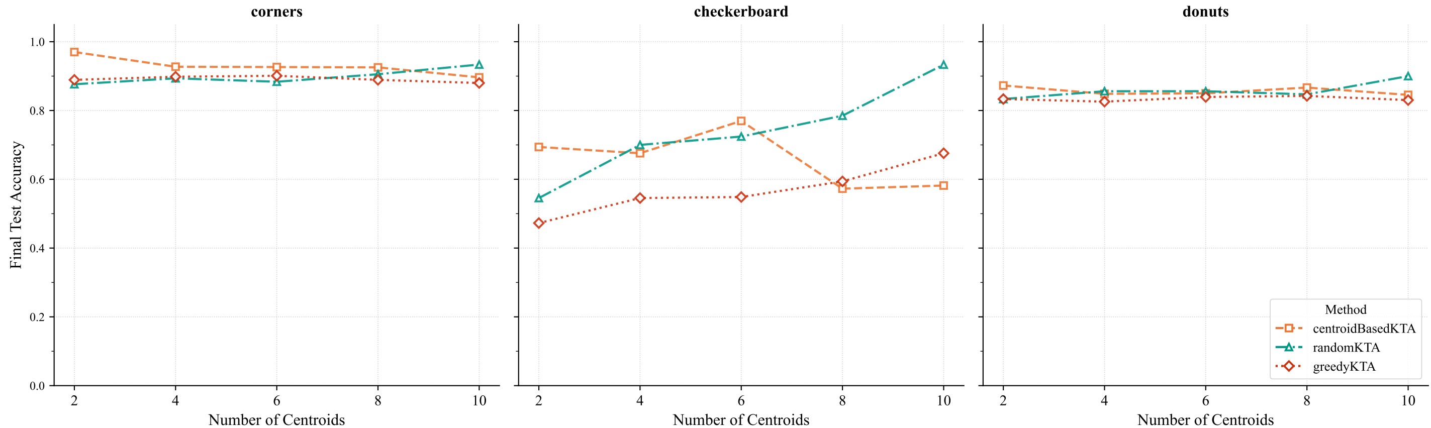
Final Test Accuracy vs. Number of Samples/Centroids
