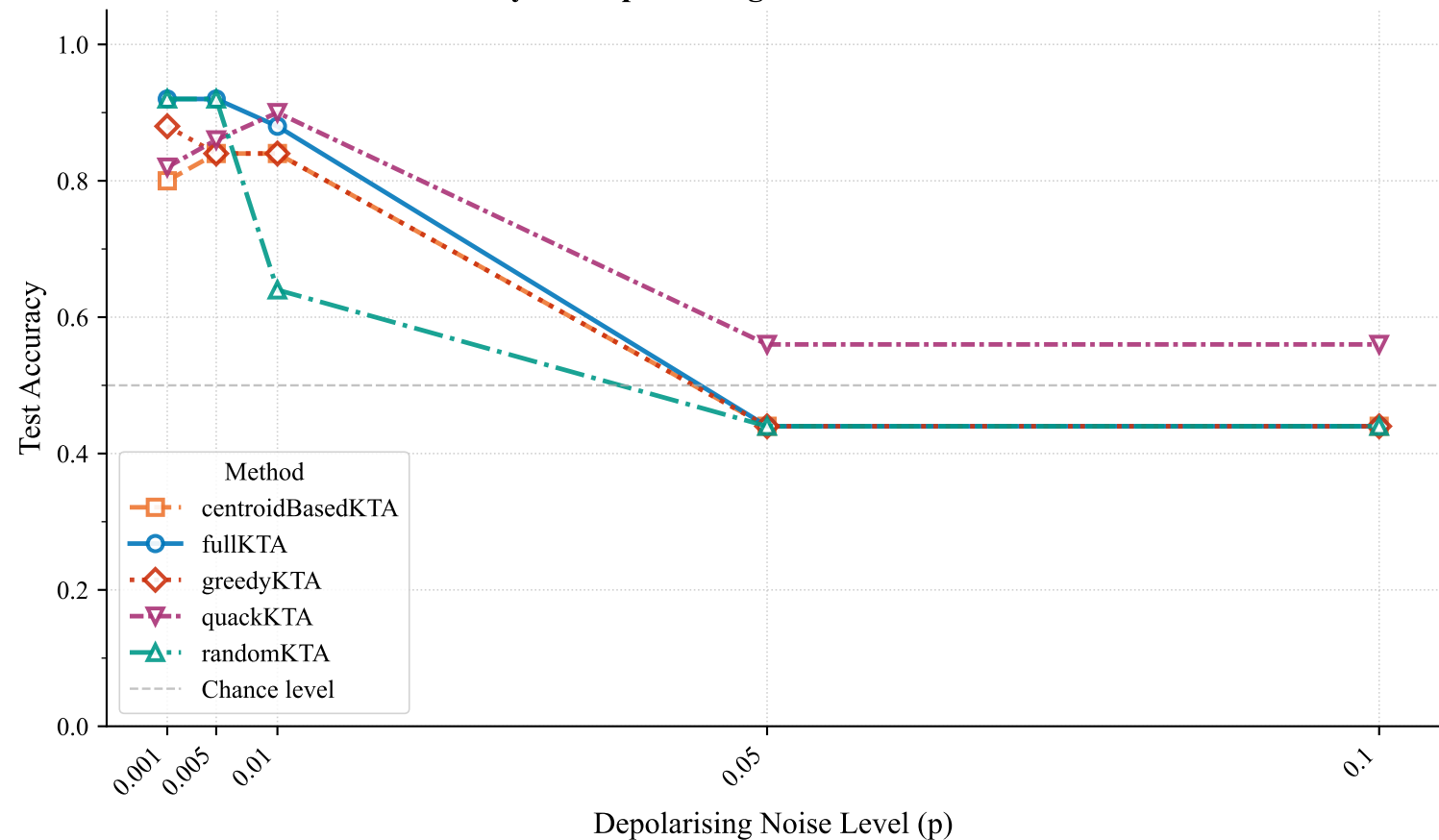
Test Accuracy vs. Depolarising Noise Level — Corners Dataset
