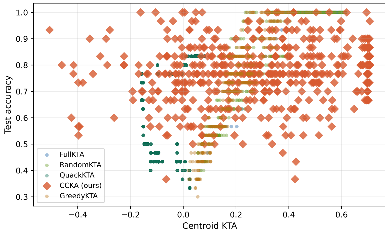
Centroid KTA vs test accuracy checkerboard
