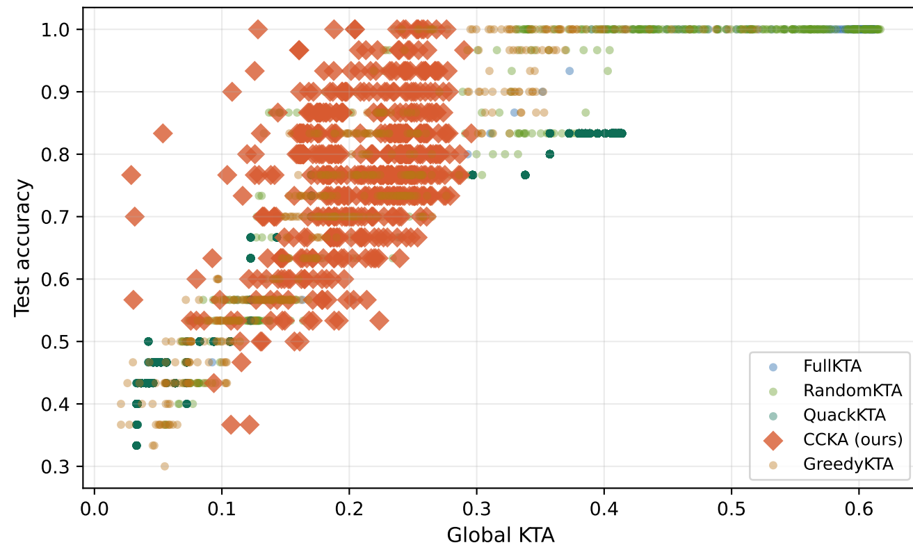
Global KTA vs test accuracy checkerboard
