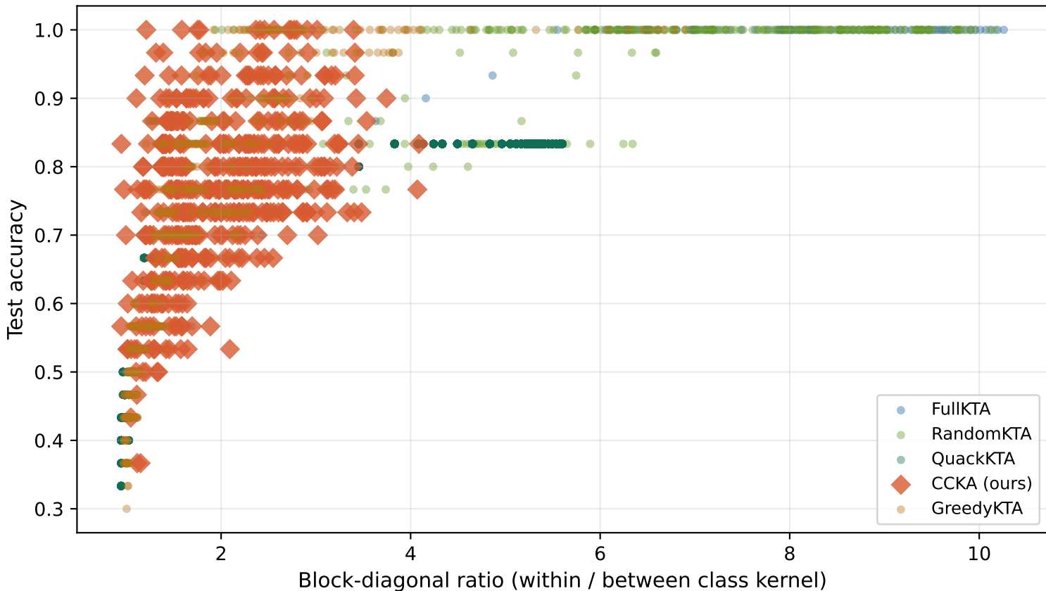
Experiment 2: Block ratio vs test accuracy — checkerboard CCKA (◆) should show high block ratio even at lower global KTA
