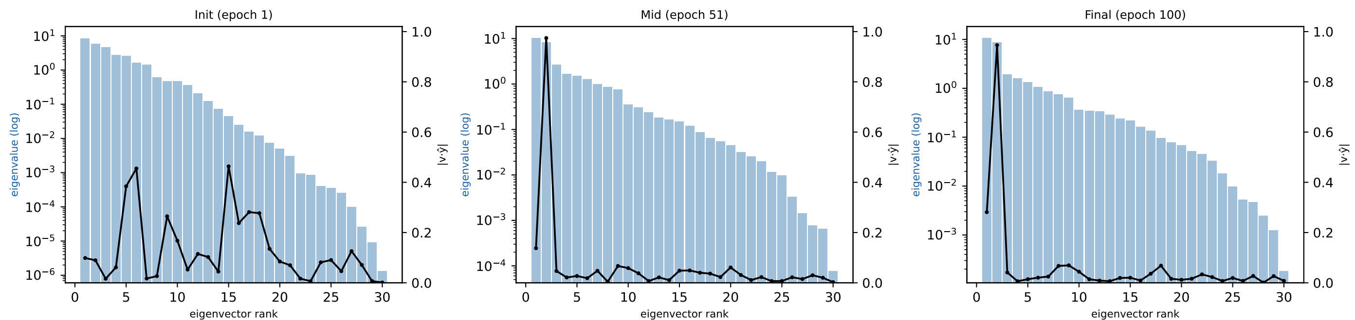
Eigenvalue spectrum (bars) + label alignment (line) — checkerboard CCKA: label alignment concentrated in few eigenvectors (low-rank)
